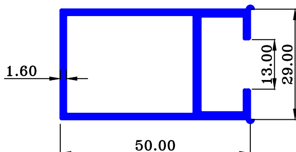
MAAN SEC.-89911 0.777 Kg/Mtr.
