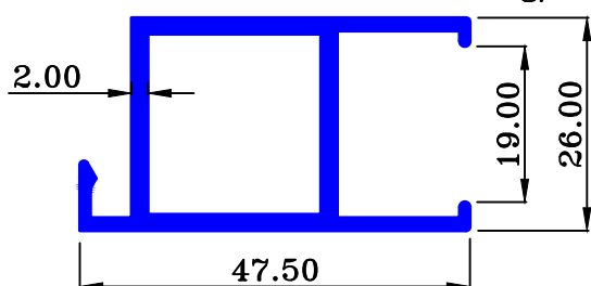
MAAN SEC.-89413 0.717 Kg/Mtr.
