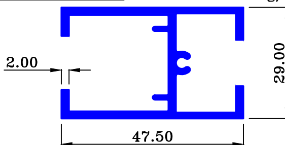
MAAN SEC.-89406 0.799 Kg/Mtr.
