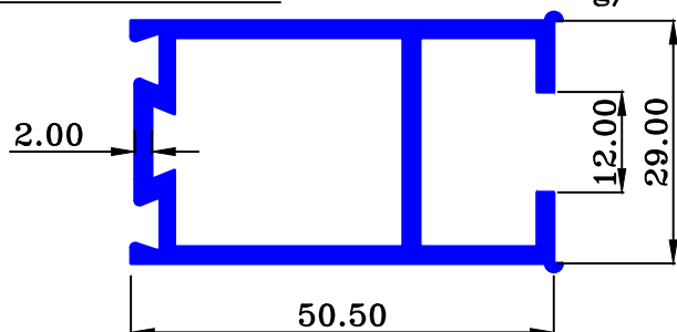
MAAN SEC.-89412 0.937 Kg/Mtr.
