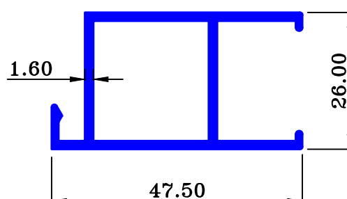
MAAN SEC.-89402 0.622 Kg/Mtr.
