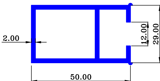
MAAN SEC.-89414 0.893 Kg/Mtr.
