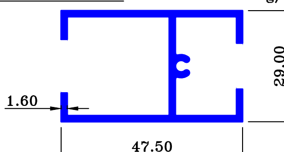
MAAN SEC.-89397 0.663 Kg/Mtr.
