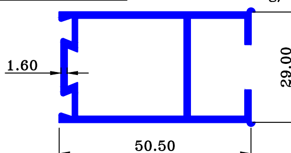
MAAN SEC.-89400 0.767 Kg/Mtr.
